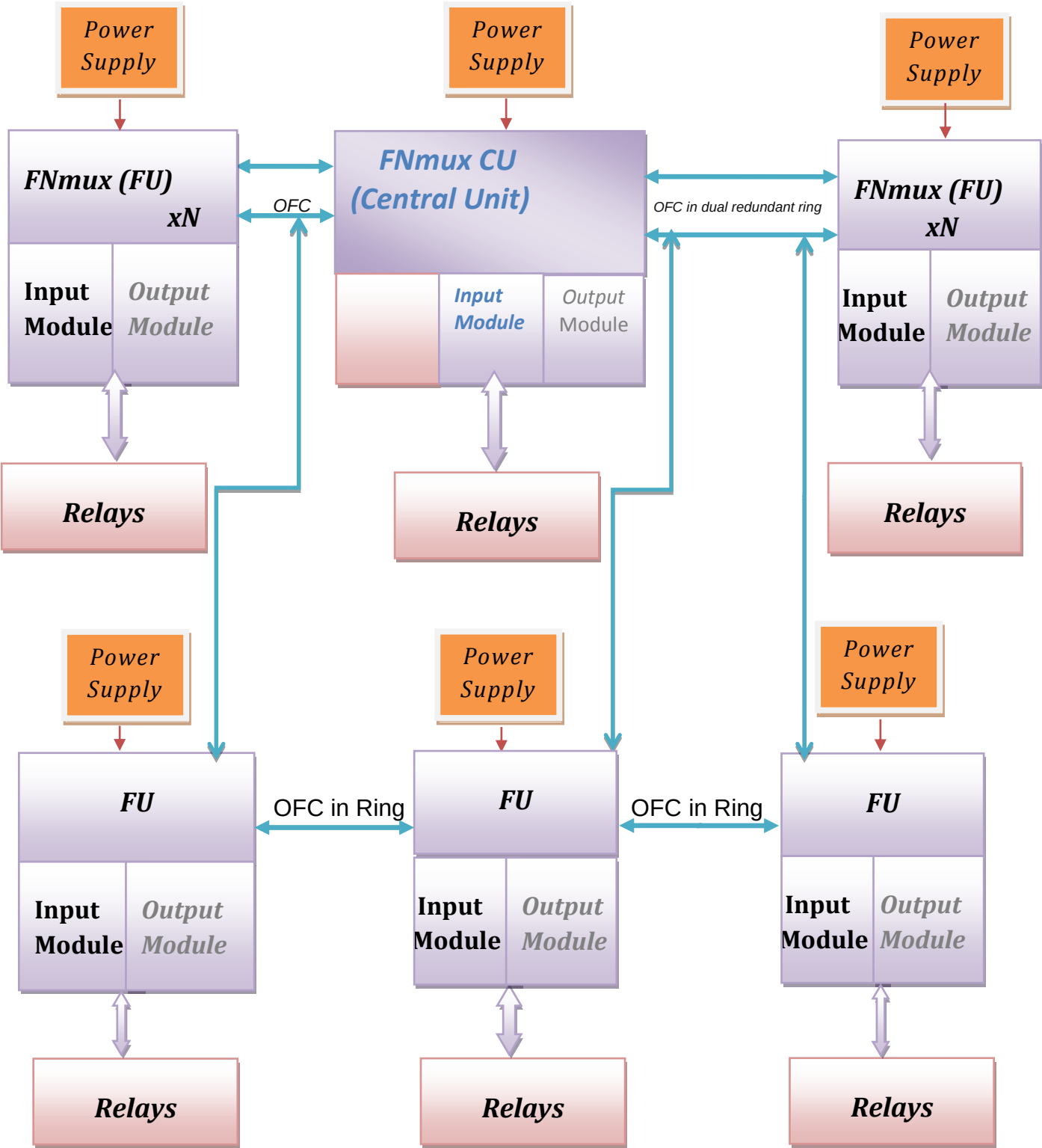
Block Working Diagram of CU with FU
